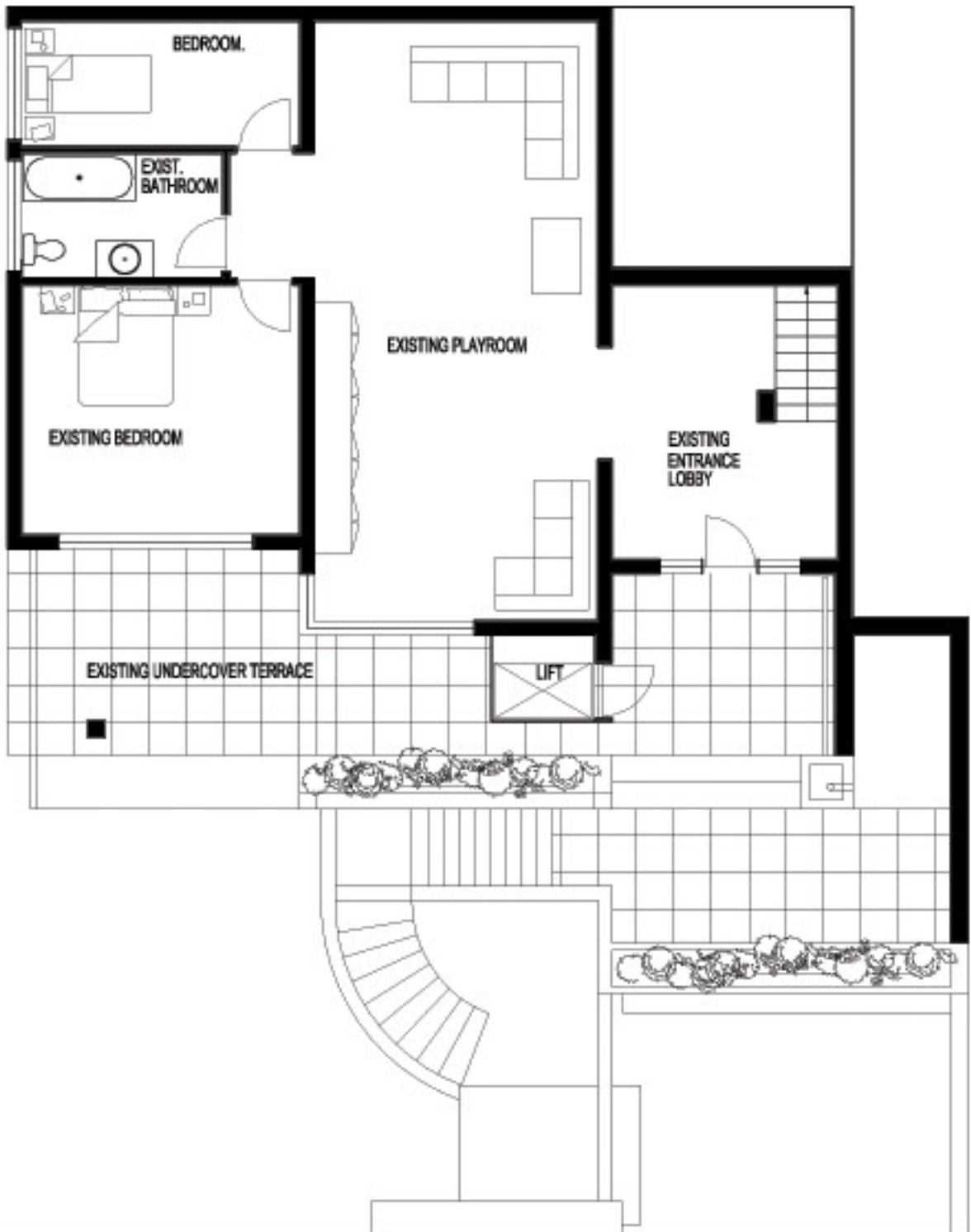
ENTRANCE LEVEL PLAN
