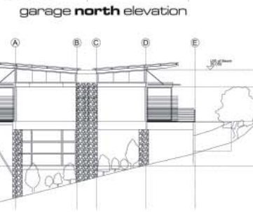
garage north elevation
