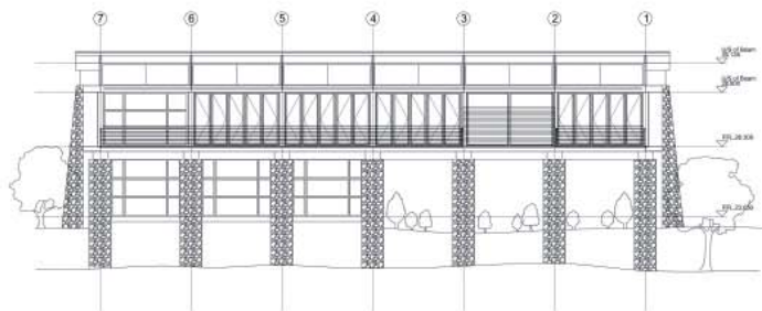
north elevation
